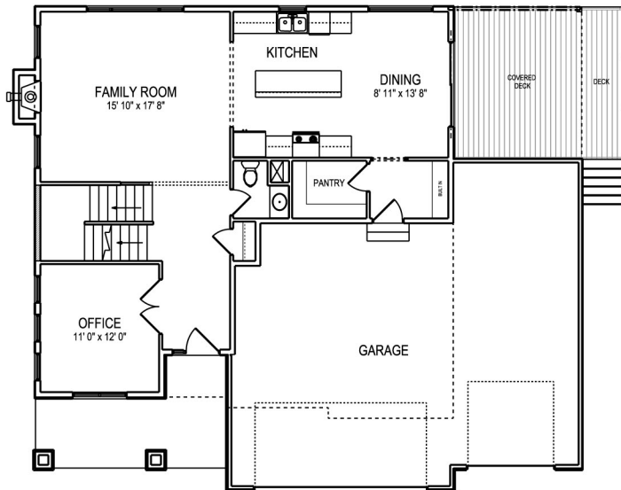
MAIN LEVEL PLAN
