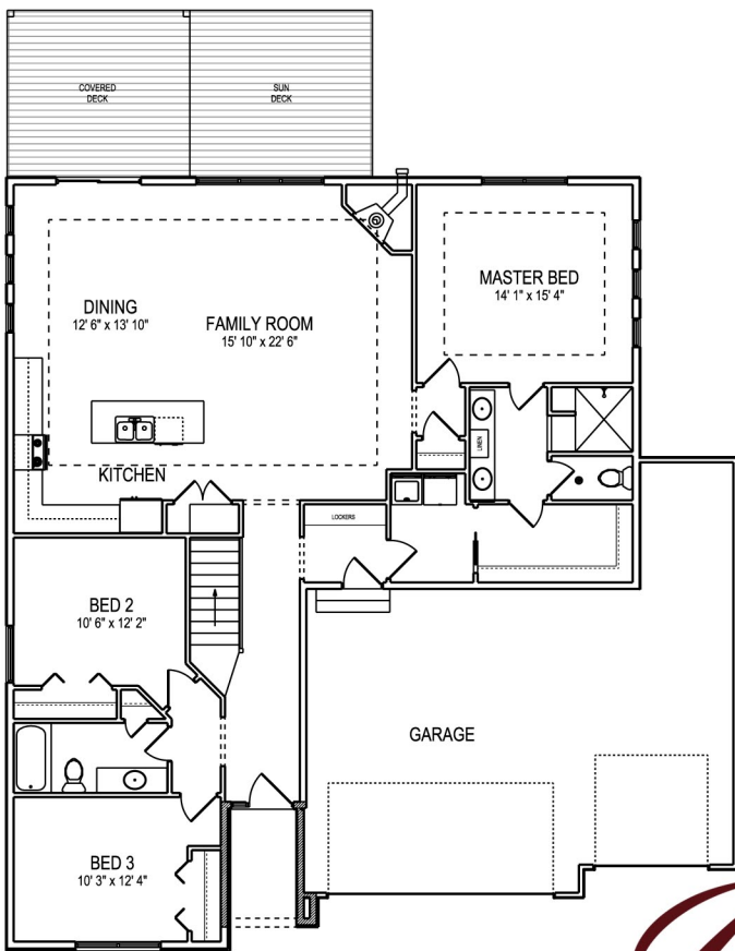
MAIN LEVEL PLAN
